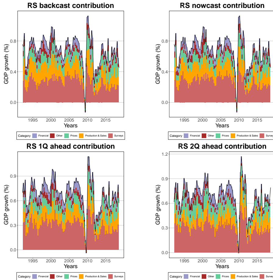
Figure 5 Contributions of the time series to random subset regression forecasts
